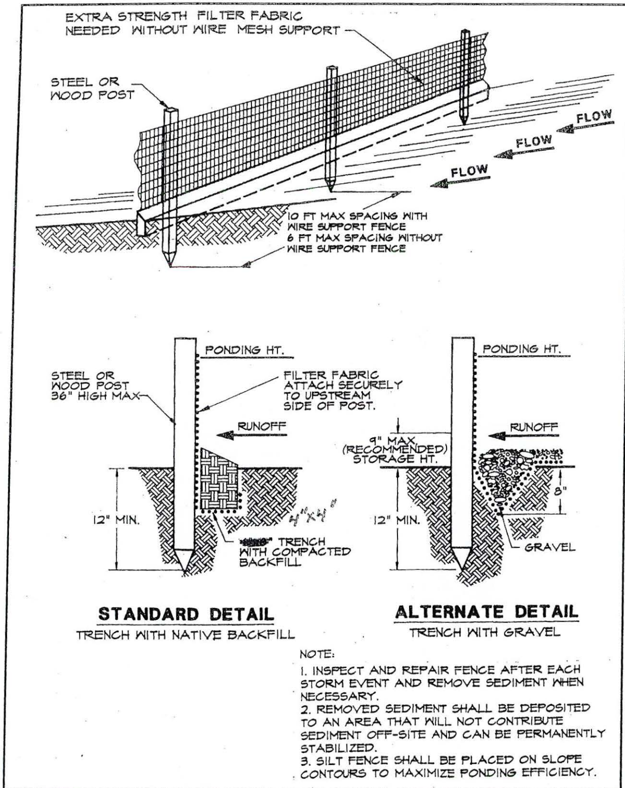
Figure 4.4a. Silt Fence
